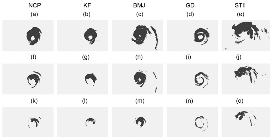
FIG. 11. Simulated Hurricane Rita precipitation patterns for rainfall values above (a)–(e) the 50th, (f)–(j) 75th, and (k)–(o) 90th percentiles. NCP, KF, BMJ, and GD are shown.
