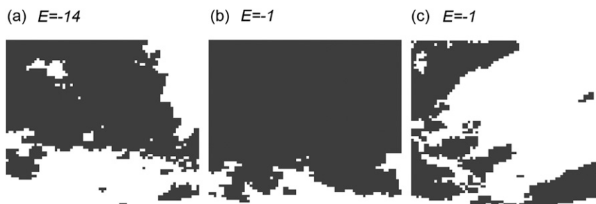
FIG. 2. The Euler number for three radar rainfall images: (a) E = -14 , (b) E = -1 , and (c) E = -1 .
