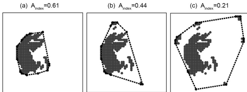
FIG. 9. The A_{\text{index}} for three example patterns: (a) A_{\text{index}} = 0.61 , (b) A_{\text{index}} = 0.44 , and (c) A_{\text{index}} = 0.21 .
