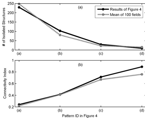
FIG. 5. (a) The number of isolated structures and (b) the connectivity indices of the patterns shown in Fig. 4.
