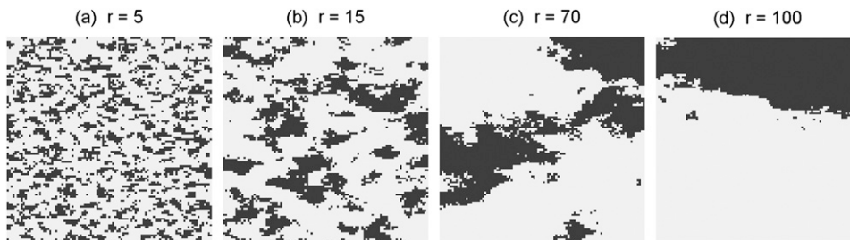
FIG. 4. Stochastically generated patterns with different correlation ranges: (a) r = 5 ; (b) r = 15 ; (c) r = 70 ; and (d) r = 100 .
