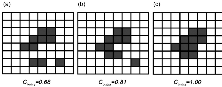
FIG. 3. The connectivity index ( C_{index} ) for three patterns.
