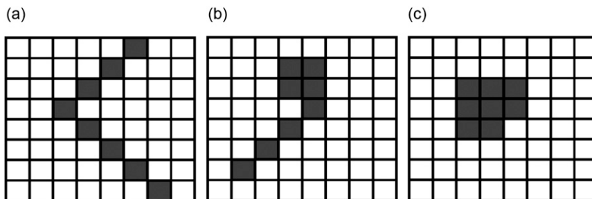
FIG. 6. Three patterns with similar Euler numbers and connectivity indices of 1.
