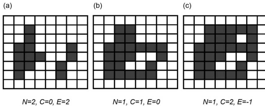
FIG. 1. Euler number for three patterns: (a) E = 2 , (b) E = 0 , and (c) E = -1 .
