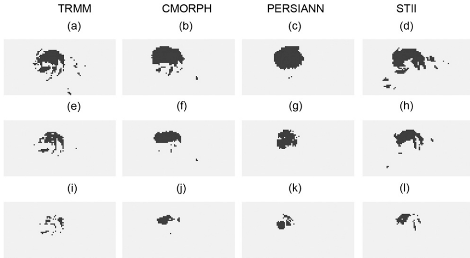
FIG. 10. The TRMM, CMORPH, PERSIANN, and stage II precipitation patterns for rainfall rates above (a)–(d) the 50th, (e)–(h) 75th, and (i)–(l) 90th percentiles.
