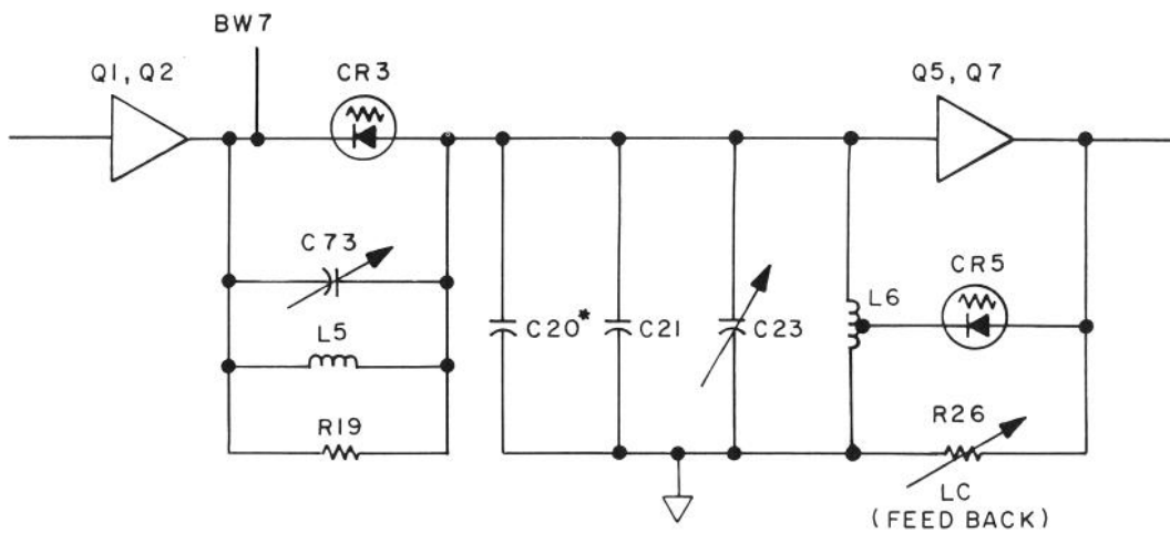
FIGURE 7-17. LC POLE, SIMPLIFIED SCHEMATIC (2147A & BELOW)
