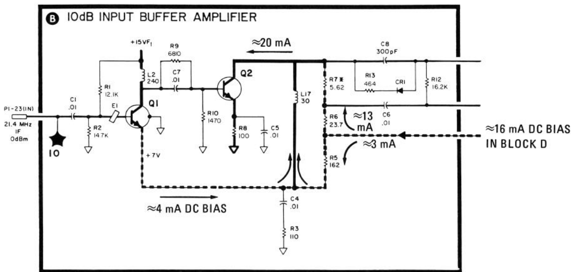
FIGURE 8-35. DC BIAS PATH DURING CRYSTAL POLE OPERATION
