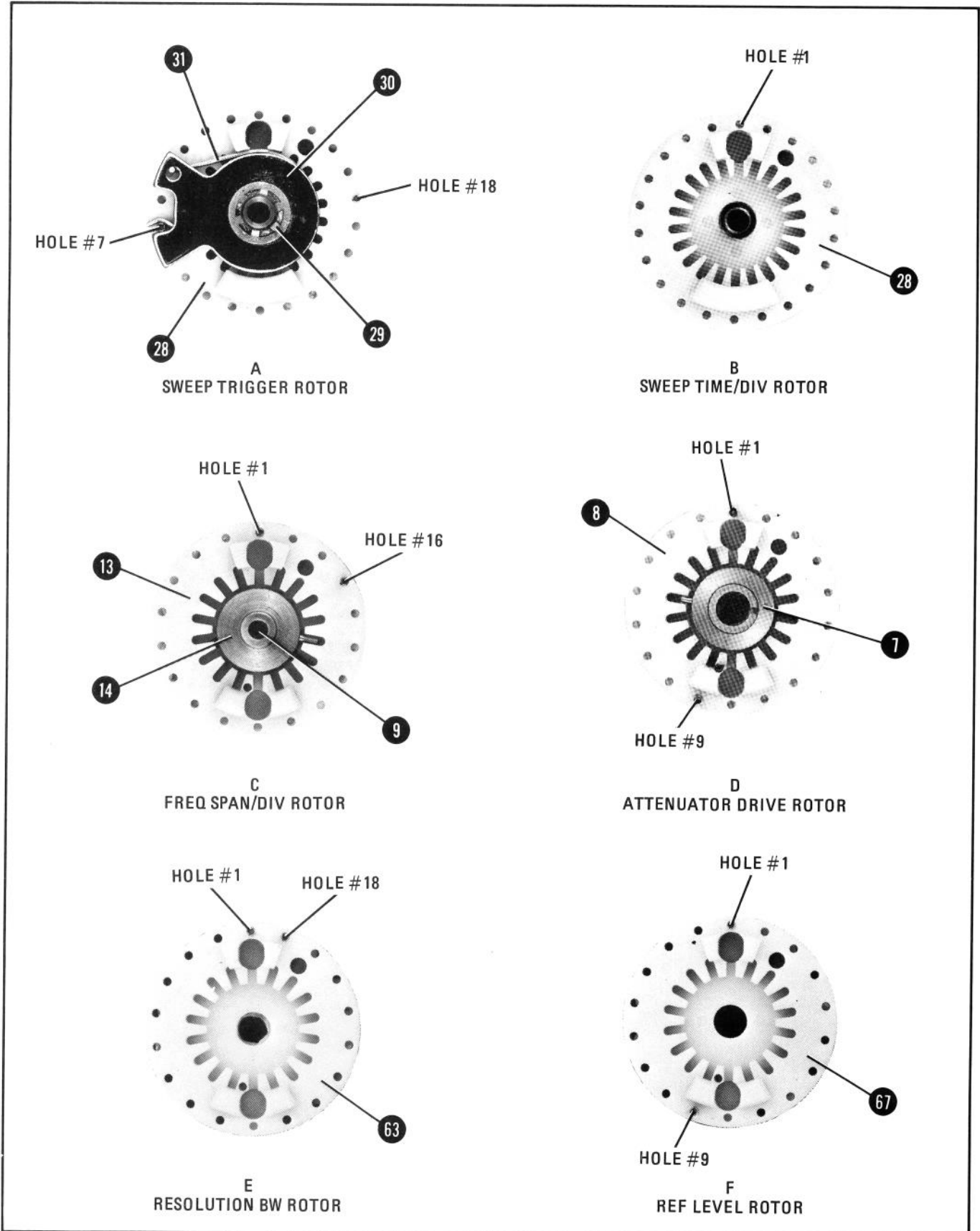
FIGURE 8-13. ROTOR ASSEMBLIES
