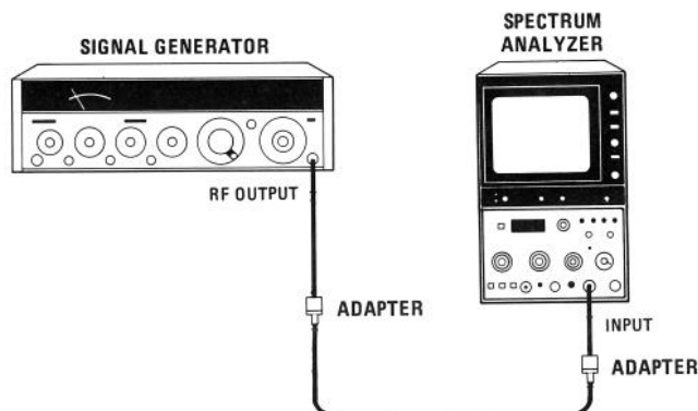
FIGURE 4-11. RESOLUTION BANDWIDTH SELECTIVITY TEST SETUP, 100 kHz TO 3 MHz
