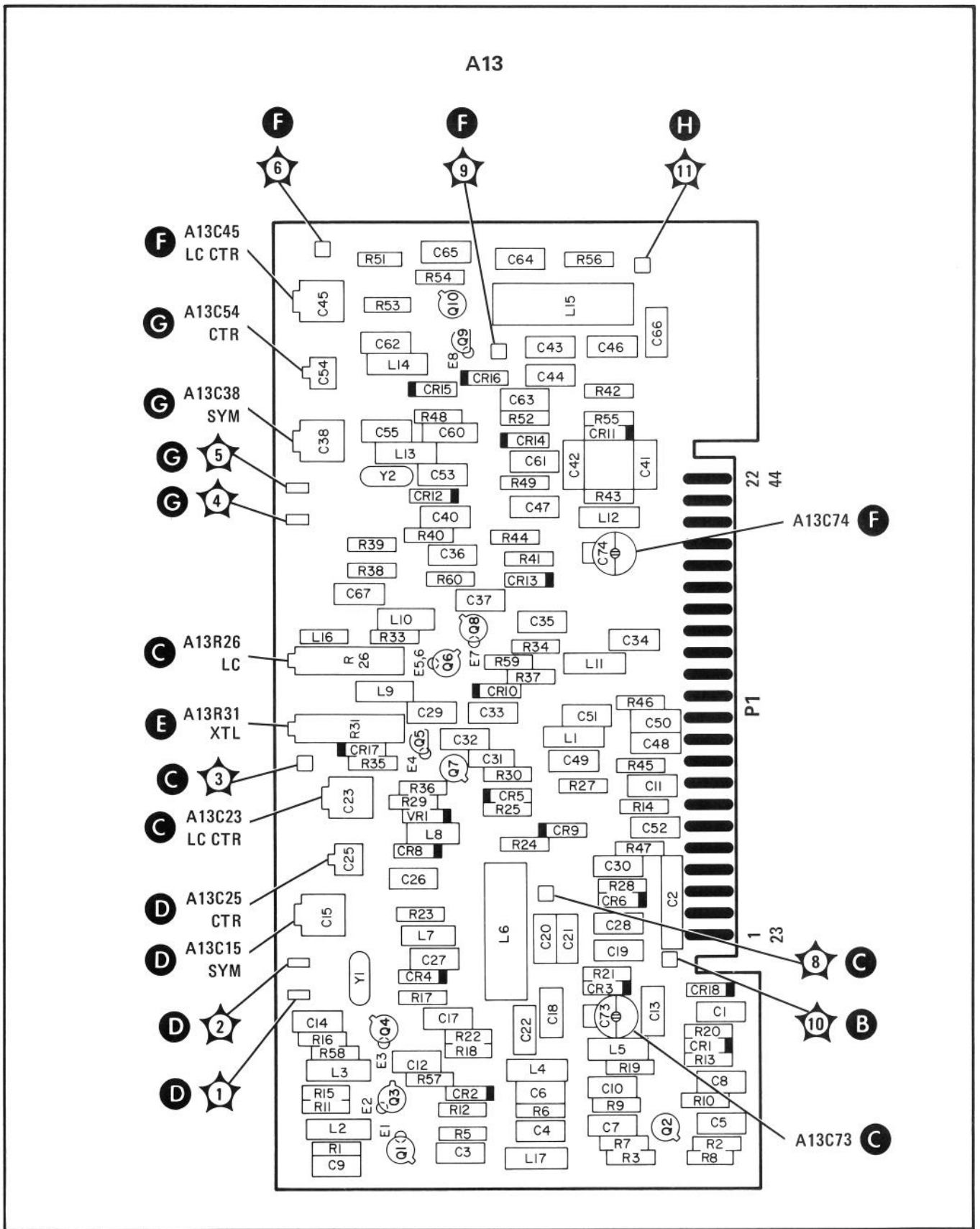
FIGURE 7-20. A13 BANDWIDTH FILTER NO. 2, COMPONENT LOCATIONS (2147A & BELOW)
